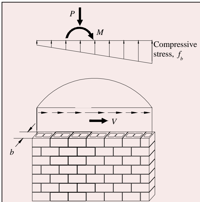
Figure 2—Unreinforced Masonry Shear Walls
